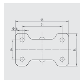
P60-95x54 Fixed castors
