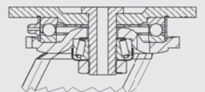
deep-groove ball thrust roller b.
