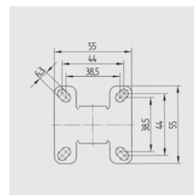
P41-55x55 Fixed castors
