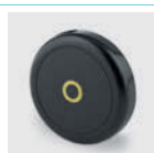
Wheel: XOI electric conductive Wheel made of Polyamide, plain bearing
