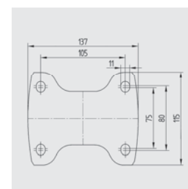
P63-137x115 Fixed castors
